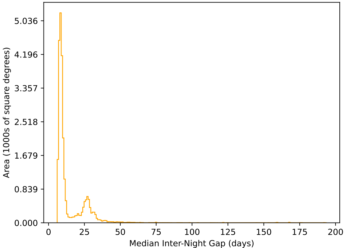
noroll_mjdp180_v3.4_10yrs All sky r band: Median Inter-Night Gap
