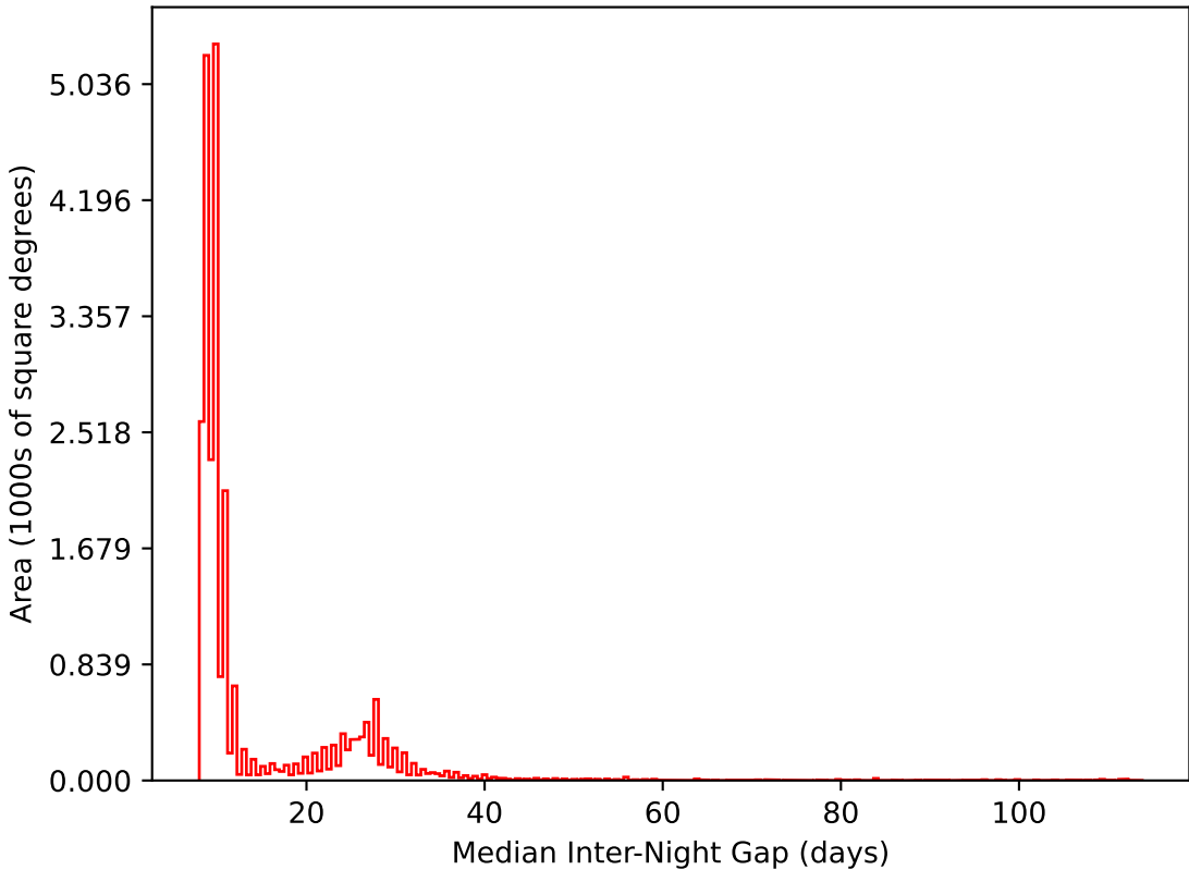
noroll_mjdp180_v3.4_10yrs All sky i band: Median Inter-Night Gap
