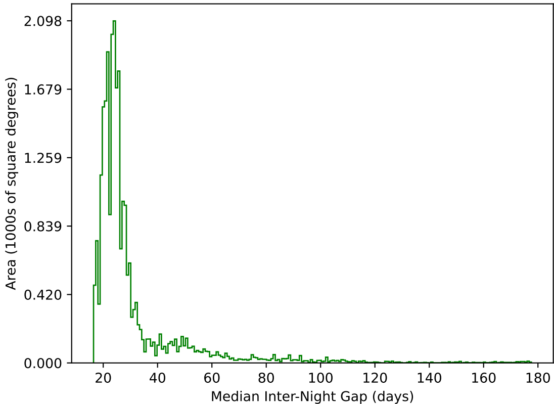
noroll_mjdp180_v3.4_10yrs All sky g band: Median Inter-Night Gap
