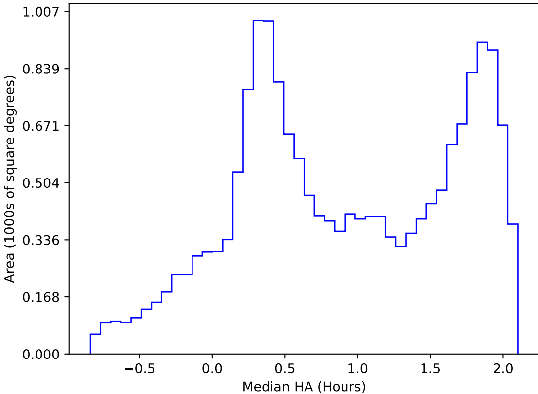
noroll_mjdp180_v3.4_10yrs WFD z band: Median HA
