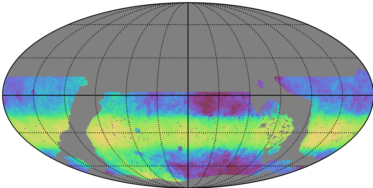
noroll_mjdp180_v3.4_10yrs WFD y band: Median HA
