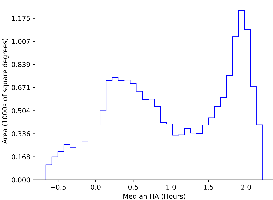
noroll_mjdp180_v3.4_10yrs WFD y band: Median HA
