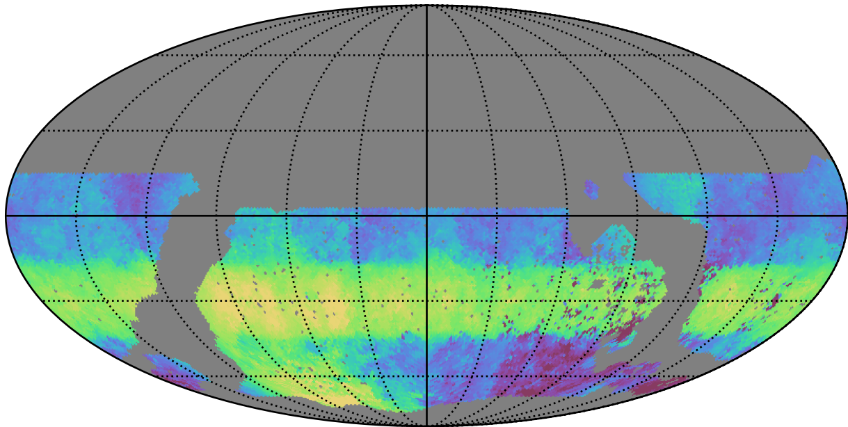
noroll_mjdp180_v3.4_10yrs WFD u band: Median HA
