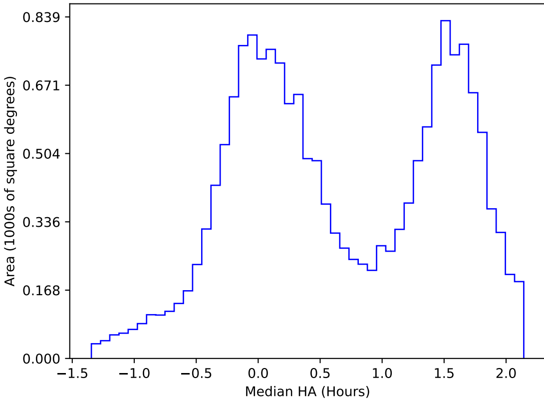
noroll_mjdp180_v3.4_10yrs WFD u band: Median HA
