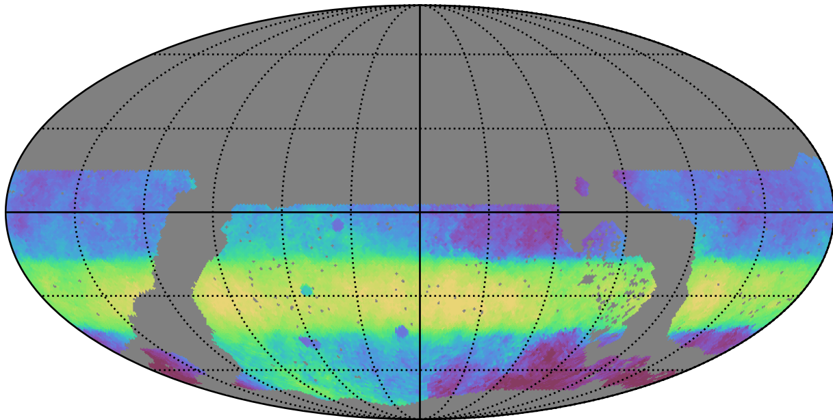
noroll_mjdp180_v3.4_10yrs WFD i band: Median HA
