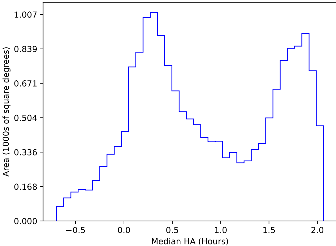
noroll_mjdp180_v3.4_10yrs WFD i band: Median HA
