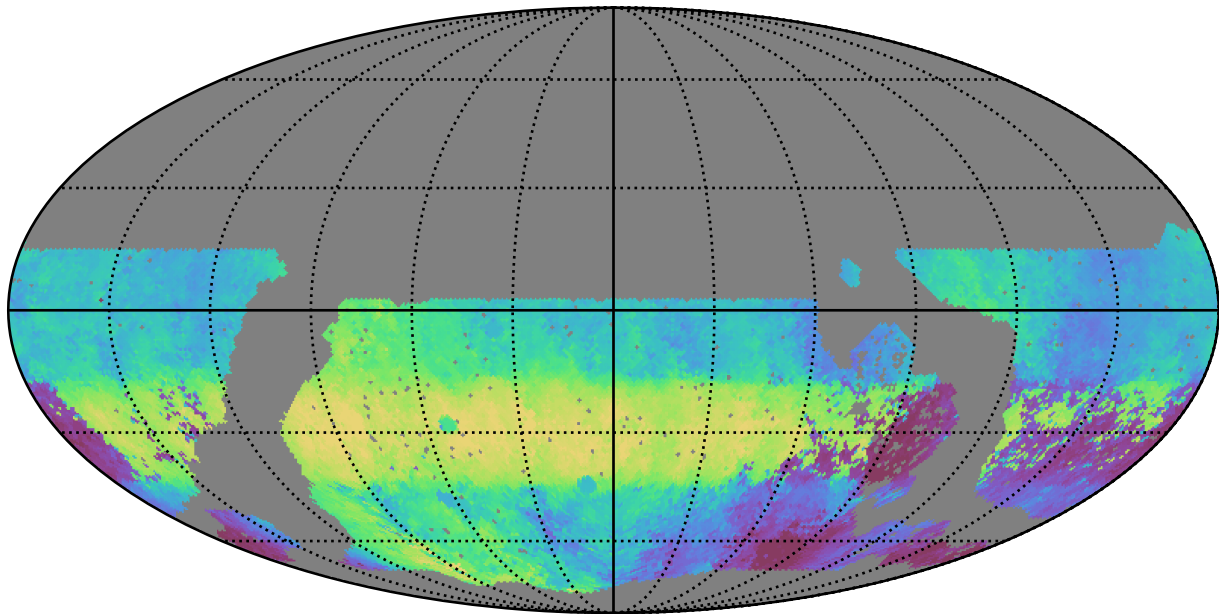
noroll_mjdp180_v3.4_10yrs WFD g band: Median HA
