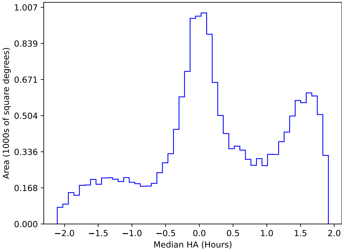
noroll_mjdp180_v3.4_10yrs WFD g band: Median HA
