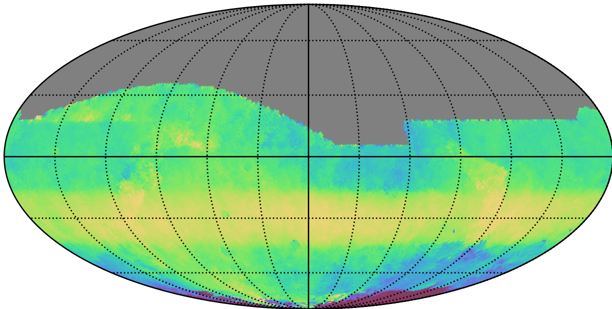
noroll_mjdp180_v3.4_10yrs All sky z band: Median HA
