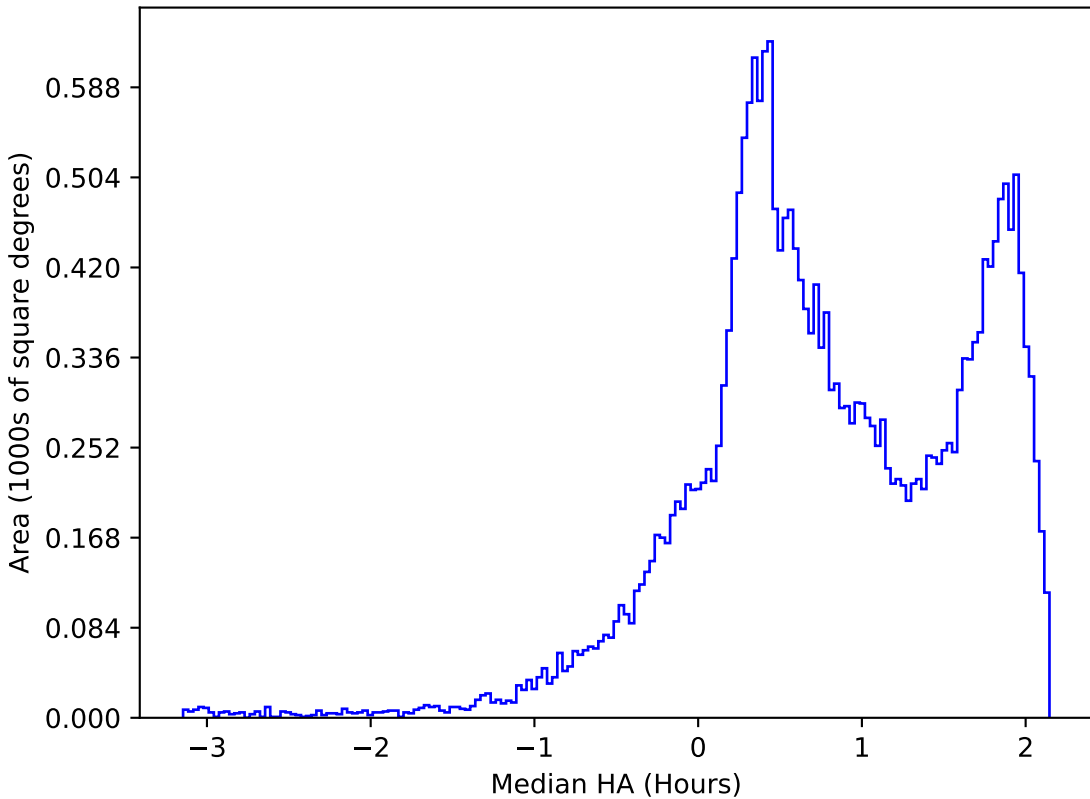
noroll_mjdp180_v3.4_10yrs All sky z band: Median HA
