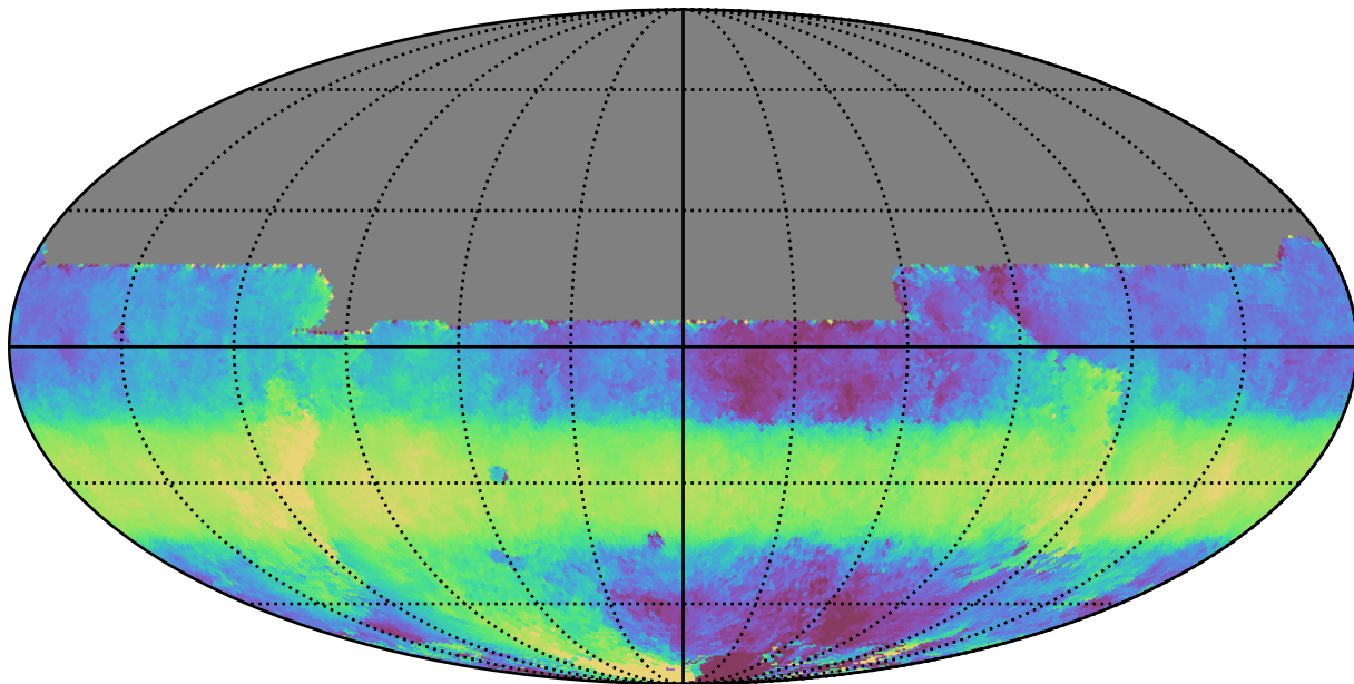
noroll_mjdp180_v3.4_10yrs All sky y band: Median HA
