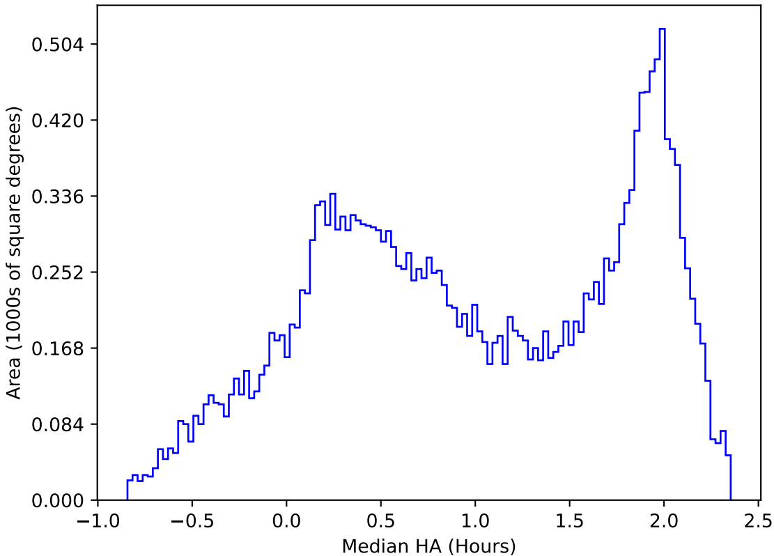
noroll_mjdp180_v3.4_10yrs All sky y band: Median HA
