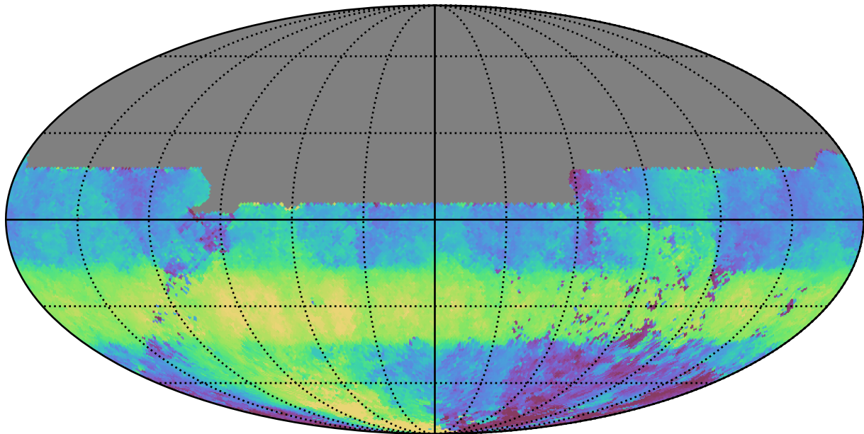
noroll_mjdp180_v3.4_10yrs All sky u band: Median HA
