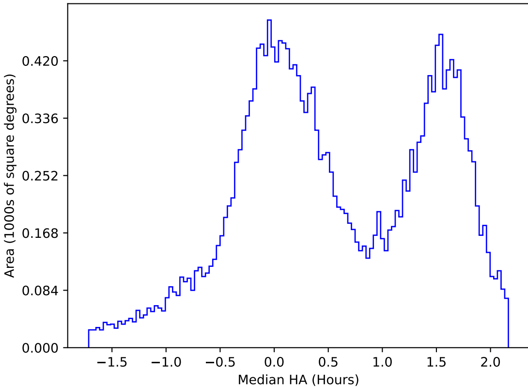
noroll_mjdp180_v3.4_10yrs All sky u band: Median HA
