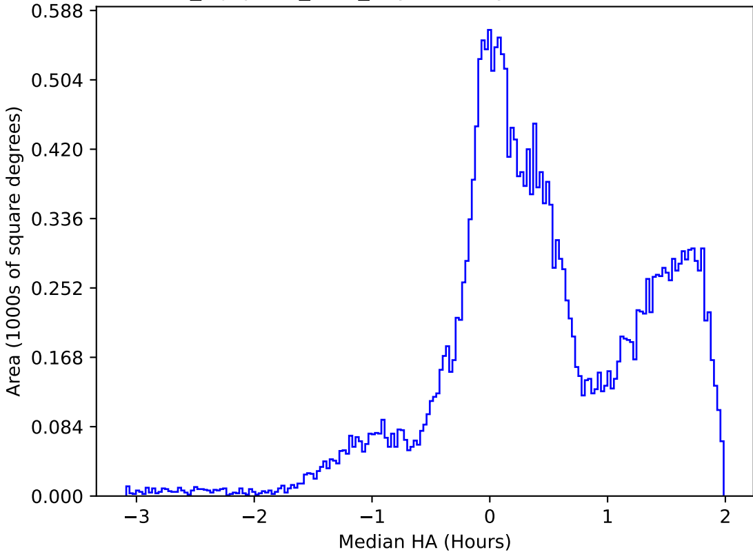
noroll_mjdp180_v3.4_10yrs All sky r band: Median HA
