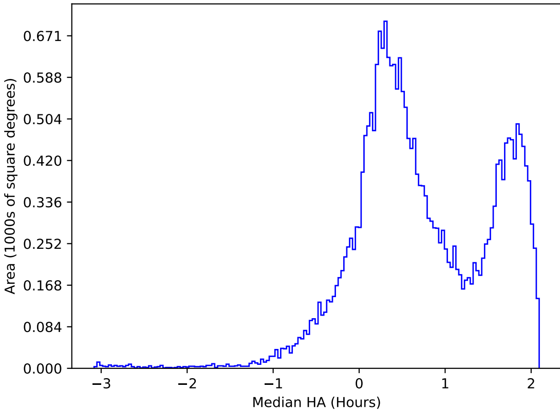
noroll_mjdp180_v3.4_10yrs All sky i band: Median HA
