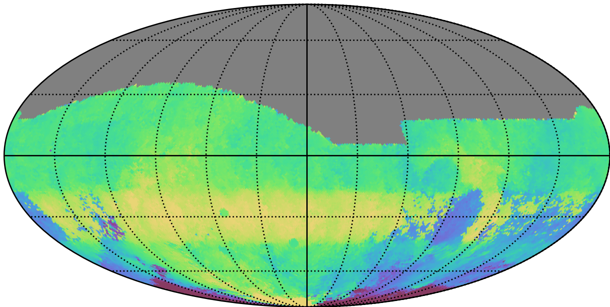
noroll_mjdp180_v3.4_10yrs All sky g band: Median HA
