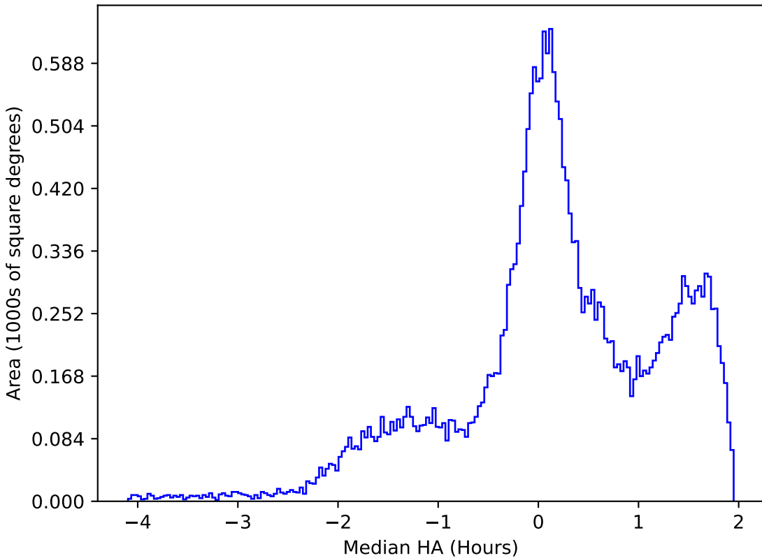
noroll_mjdp180_v3.4_10yrs All sky g band: Median HA
