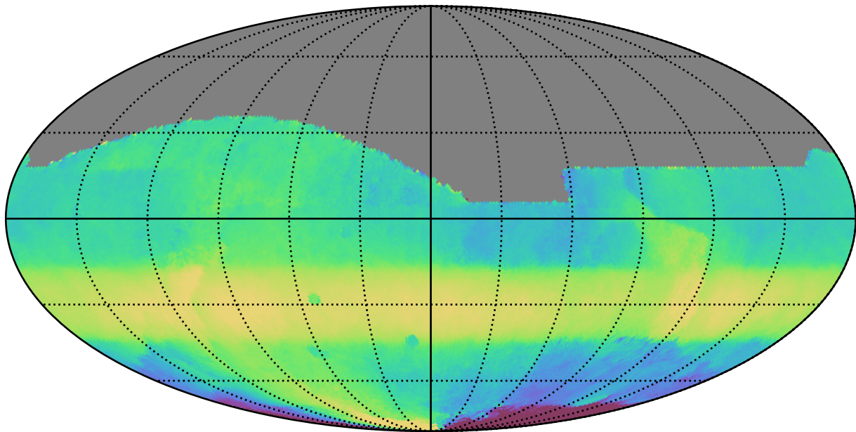
noroll_mjdp180_v3.4_10yrs All sky all bands: Median HA
