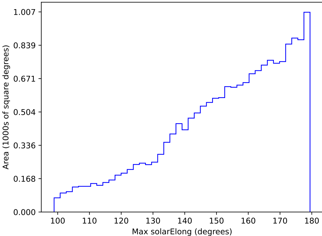
noroll_mjdp180_v3.4_10yrs WFD z band: Max solarElong
