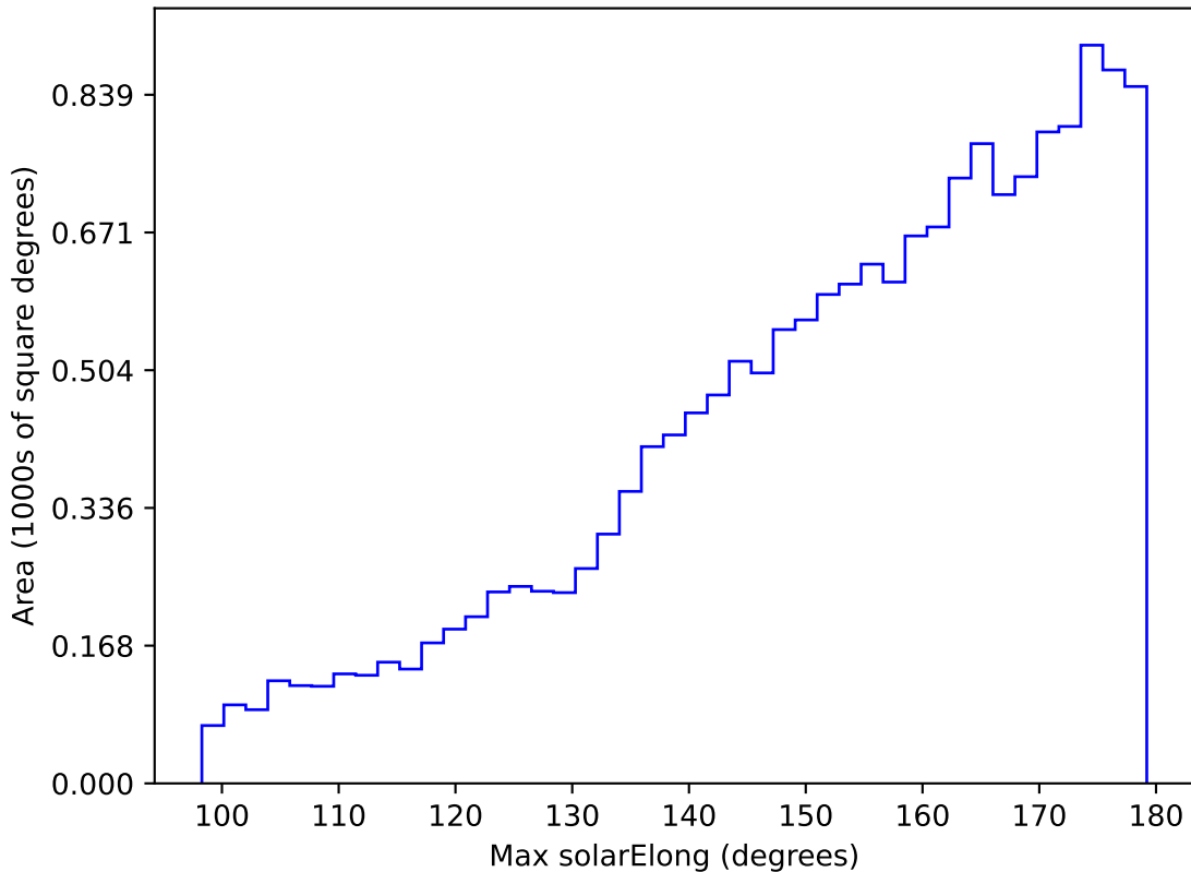
noroll_mjdp180_v3.4_10yrs WFD g band: Max solarElong
