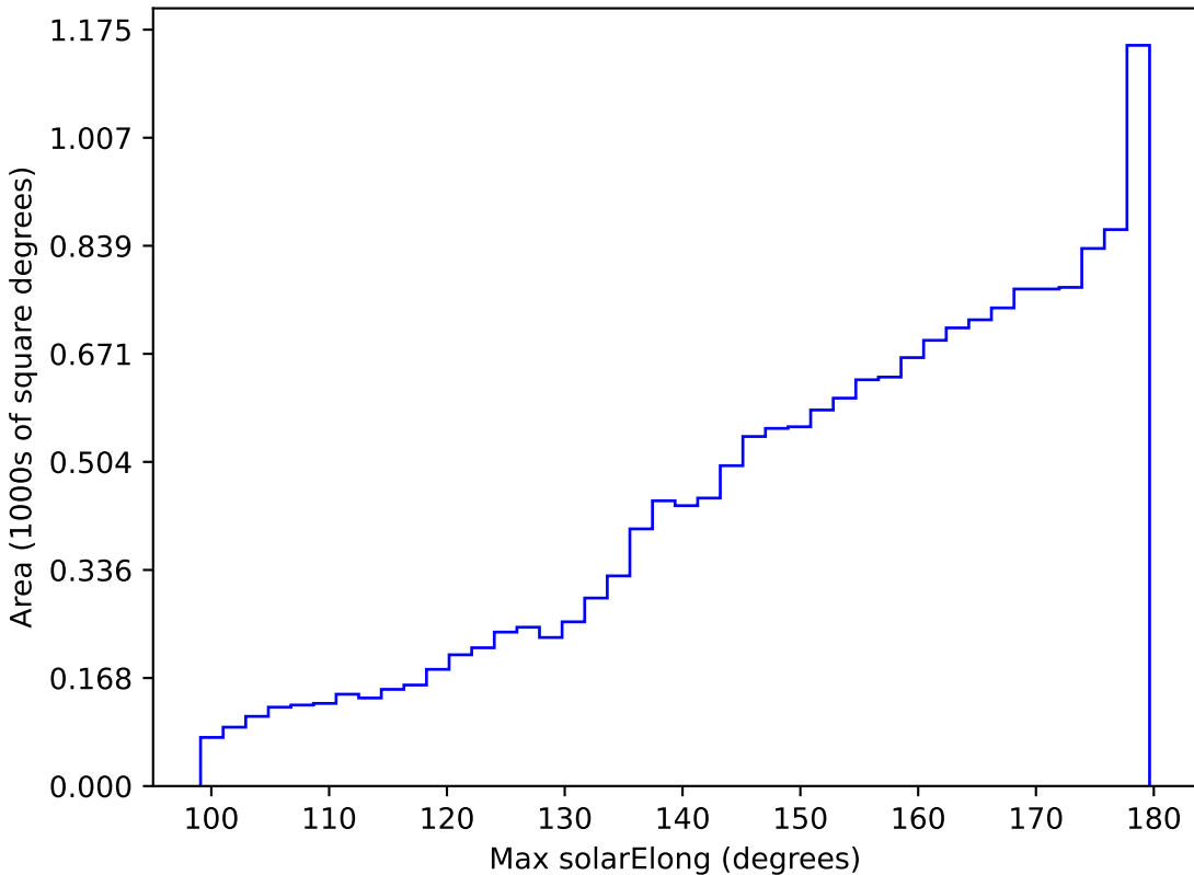
noroll_mjdp180_v3.4_10yrs WFD all bands: Max solarElong
