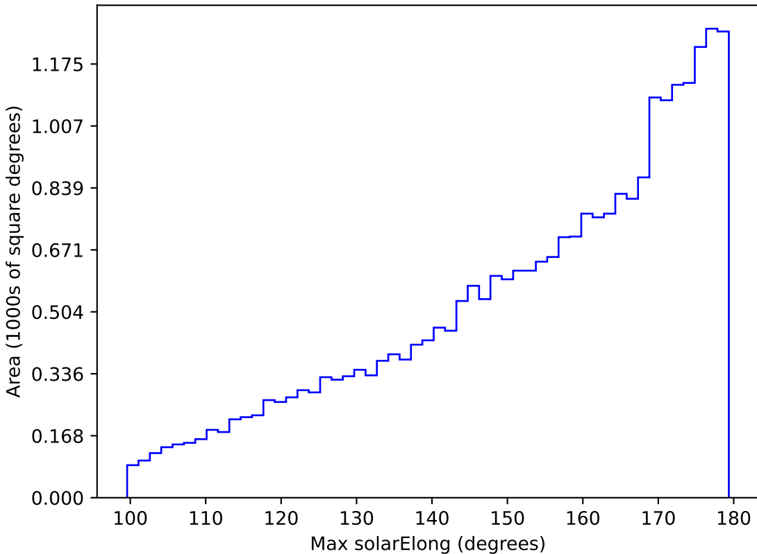
noroll_mjdp180_v3.4_10yrs All sky z band: Max solarElong
