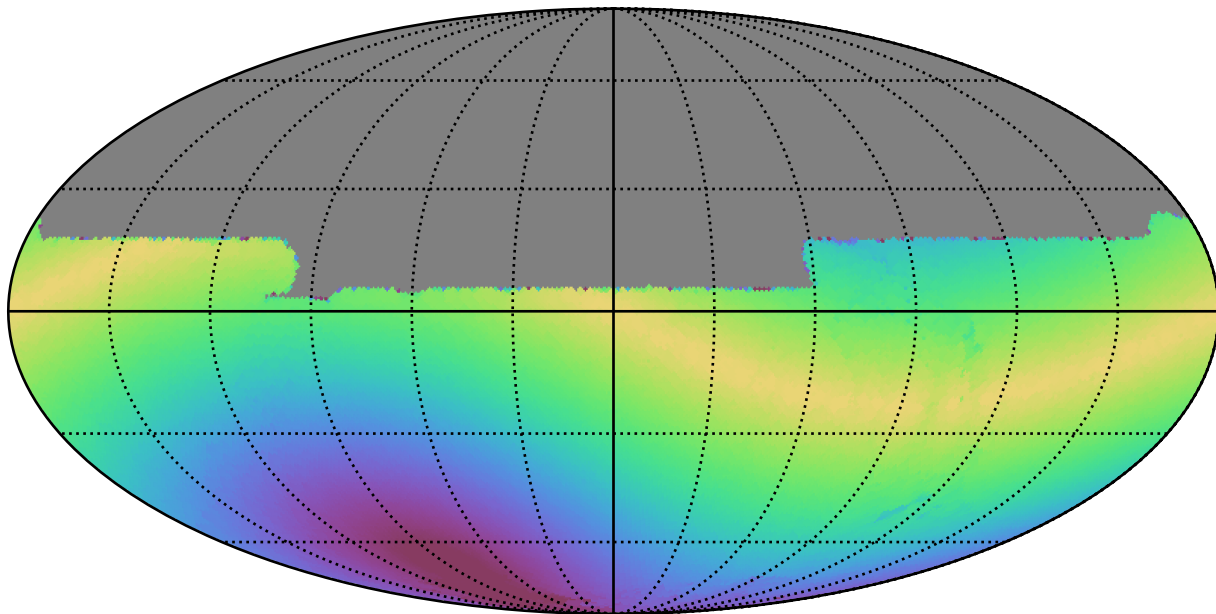
noroll_mjdp180_v3.4_10yrs All sky y band: Max solarElong
