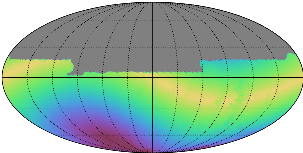
noroll_mjdp180_v3.4_10yrs All sky u band: Max solarElong
