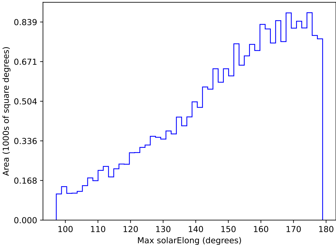
noroll_mjdp180_v3.4_10yrs All sky u band: Max solarElong
