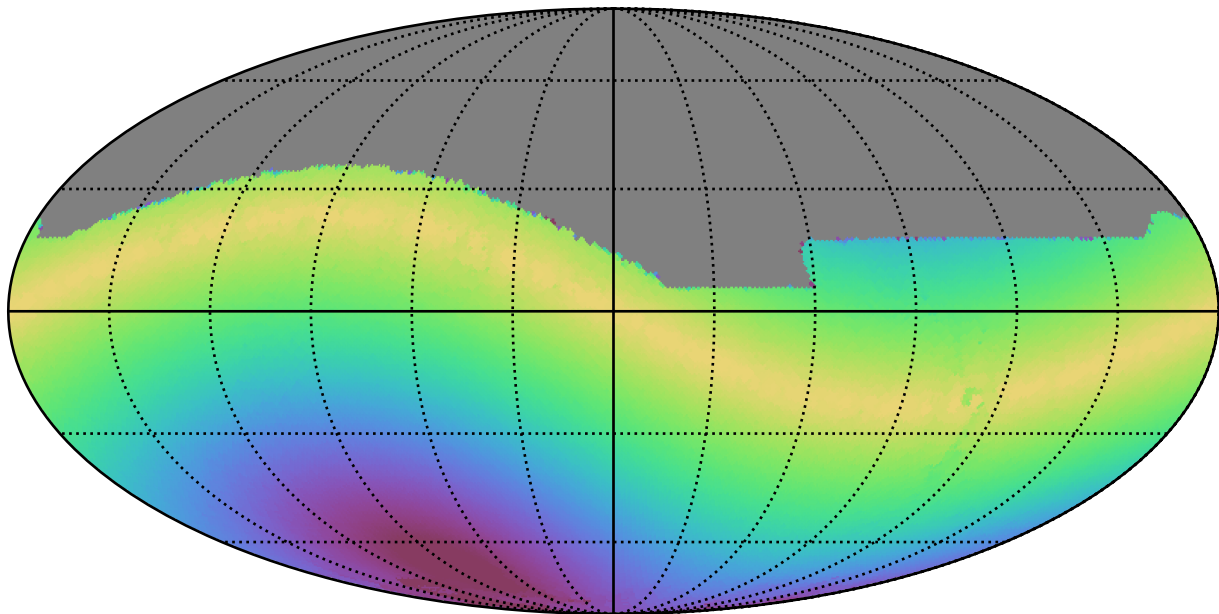
noroll_mjdp180_v3.4_10yrs All sky r band: Max solarElong
