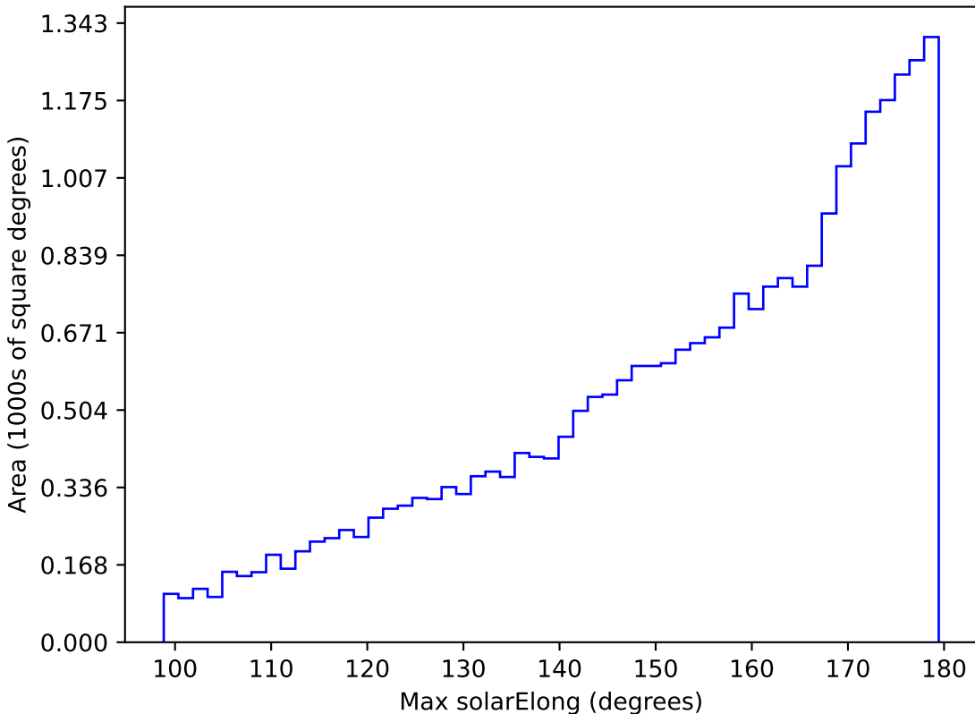
noroll_mjdp180_v3.4_10yrs All sky r band: Max solarElong
