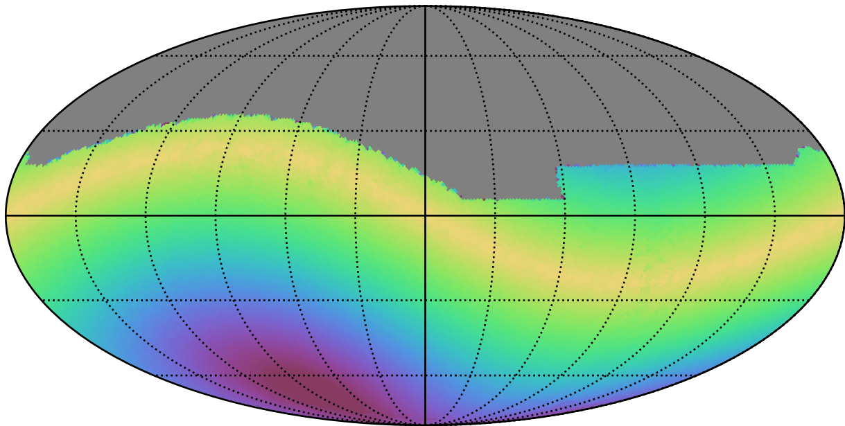
noroll_mjdp180_v3.4_10yrs All sky i band: Max solarElong
