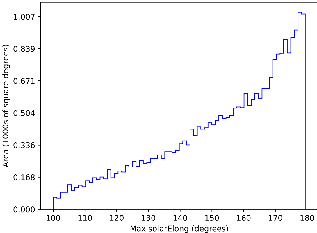
noroll_mjdp180_v3.4_10yrs All sky i band: Max solarElong
