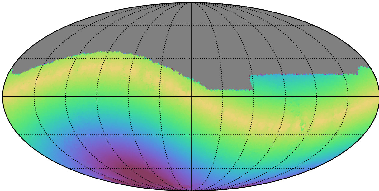
noroll_mjdp180_v3.4_10yrs All sky g band: Max solarElong
