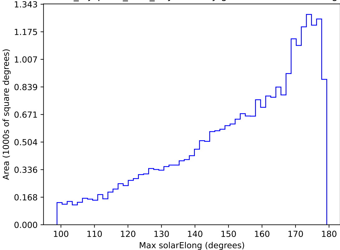
noroll_mjdp180_v3.4_10yrs All sky g band: Max solarElong
