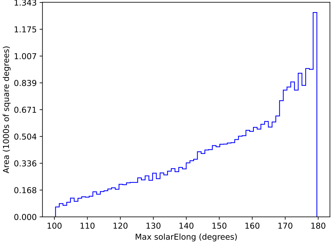
noroll_mjdp180_v3.4_10yrs All sky all bands: Max solarElong
