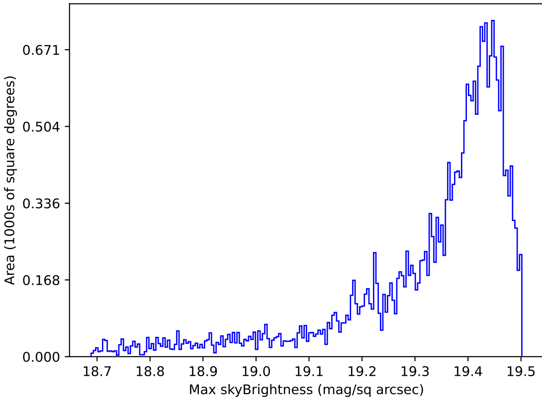
noroll_mjdp180_v3.4_10yrs Yr 1 z band: Max skyBrightness
