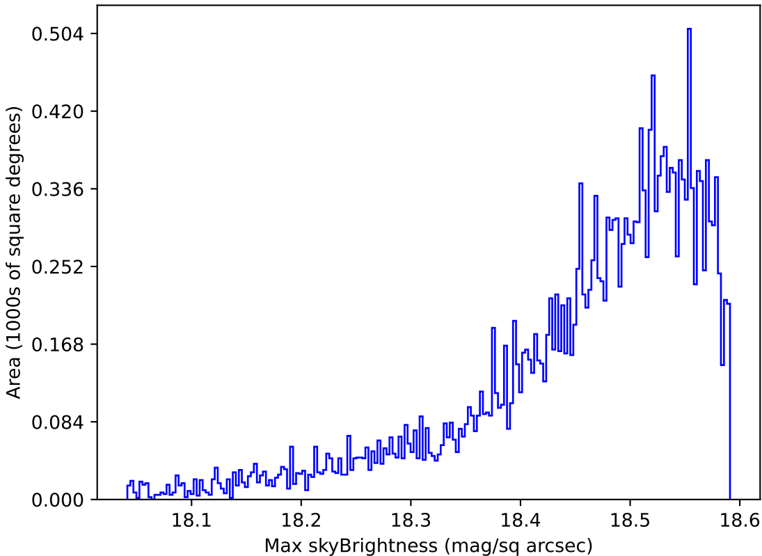
noroll_mjdp180_v3.4_10yrs Yr 1 y band: Max skyBrightness
