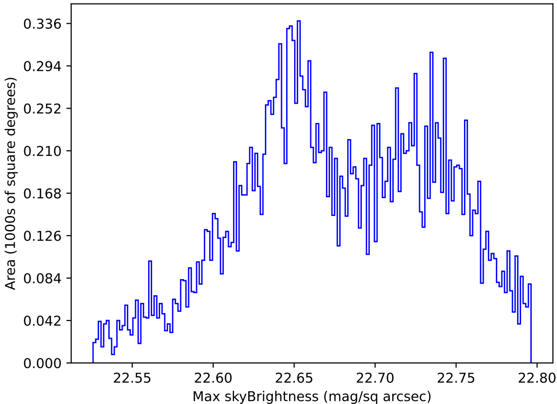
noroll_mjdp180_v3.4_10yrs Yr 1 u band: Max skyBrightness
