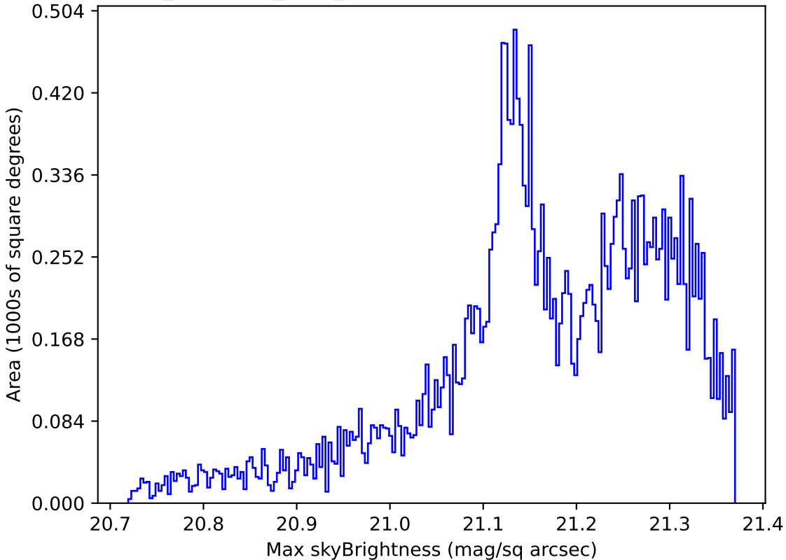
noroll_mjdp180_v3.4_10yrs Yr 1 r band: Max skyBrightness
