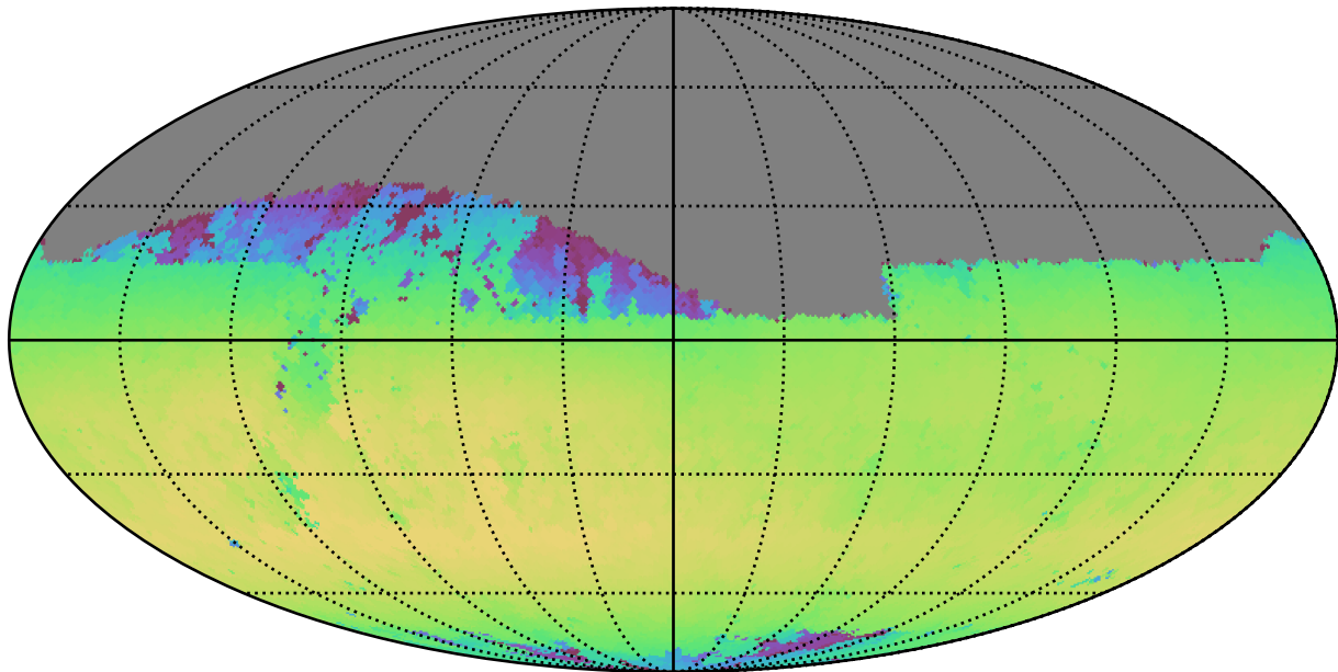
noroll_mjdp180_v3.4_10yrs Yr 1 i band: Max skyBrightness
