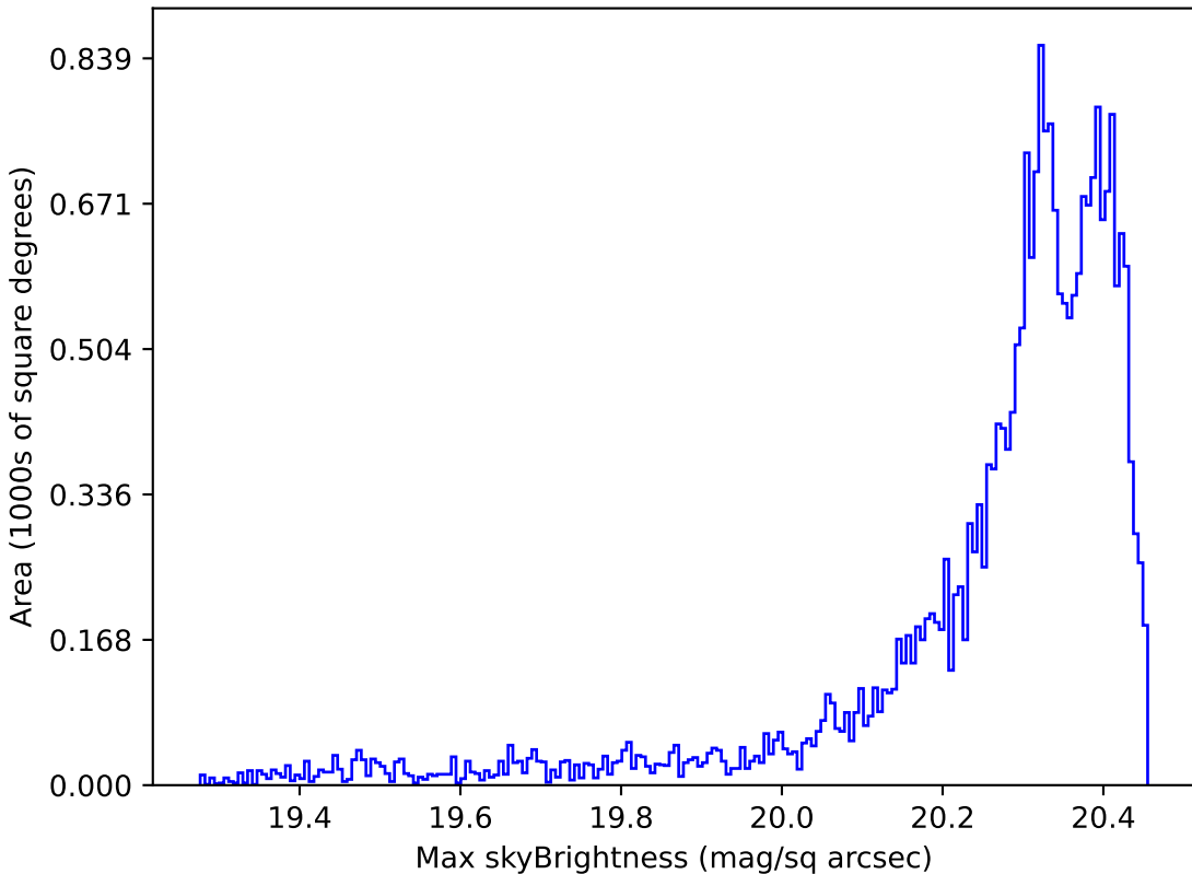
noroll_mjdp180_v3.4_10yrs Yr 1 i band: Max skyBrightness
