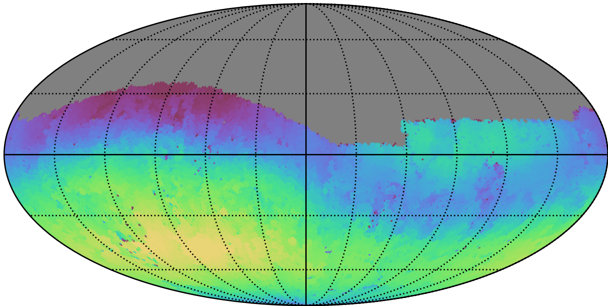
noroll_mjdp180_v3.4_10yrs Yr 1 g band: Max skyBrightness
