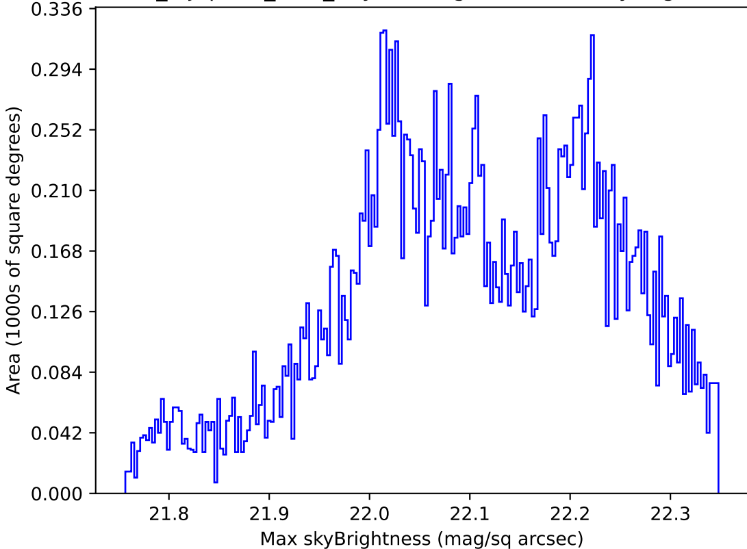
noroll_mjdp180_v3.4_10yrs Yr 1 g band: Max skyBrightness
