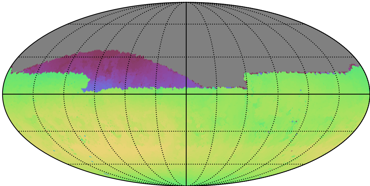
noroll_mjdp180_v3.4_10yrs Yr 1 all bands: Max skyBrightness
