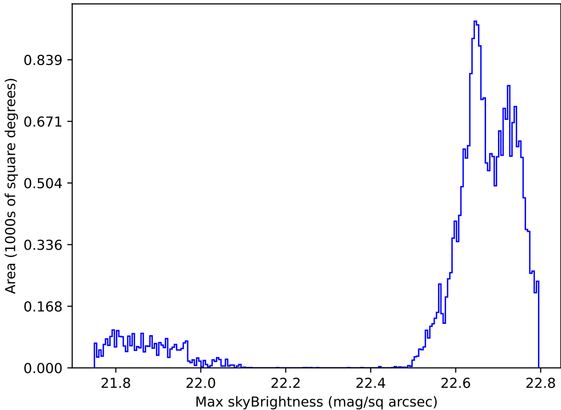
noroll_mjdp180_v3.4_10yrs Yr 1 all bands: Max skyBrightness
