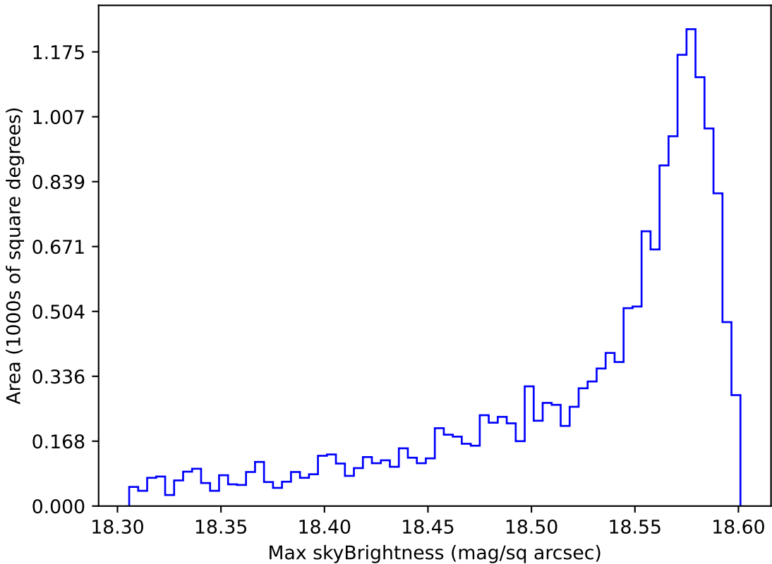
noroll_mjdp180_v3.4_10yrs WFD y band: Max skyBrightness
