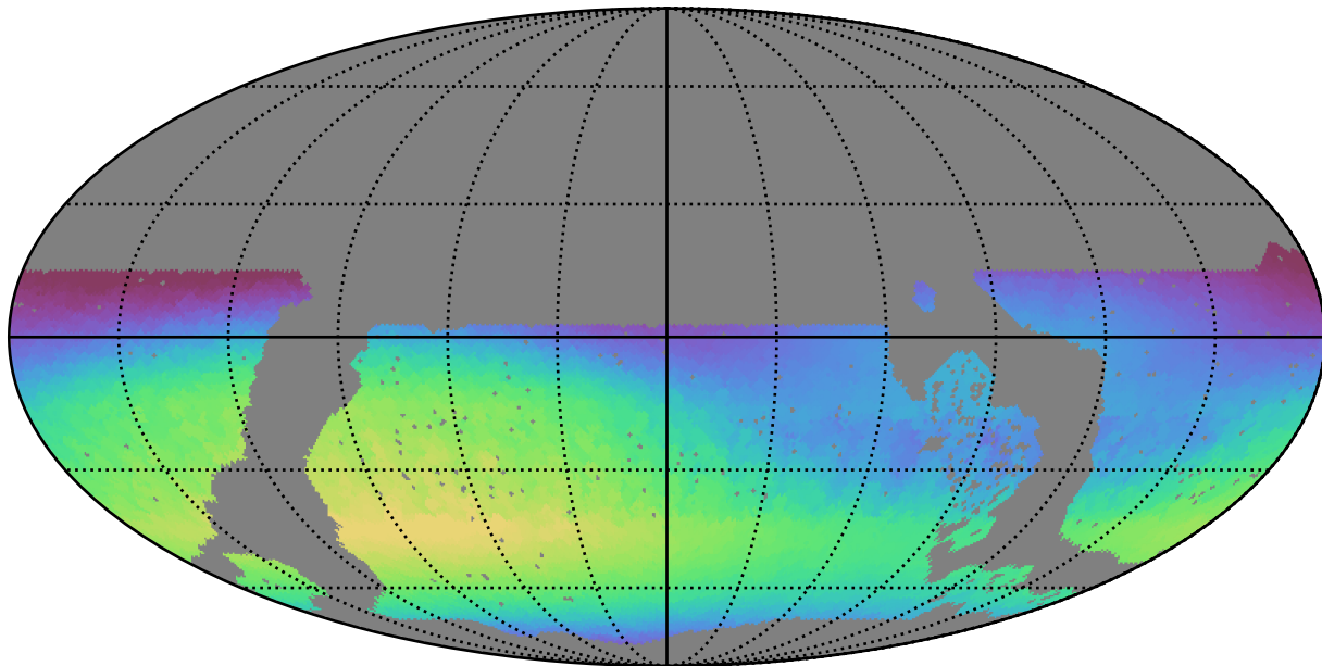
noroll_mjdp180_v3.4_10yrs WFD u band: Max skyBrightness
