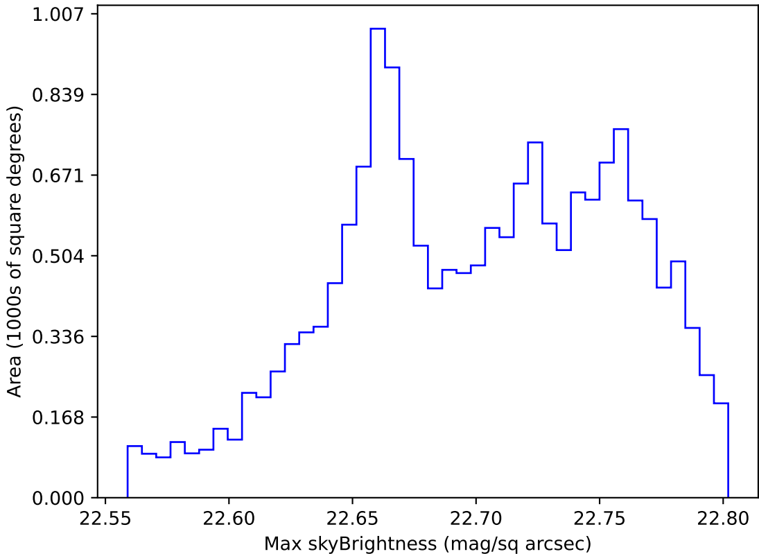
noroll_mjdp180_v3.4_10yrs WFD u band: Max skyBrightness
